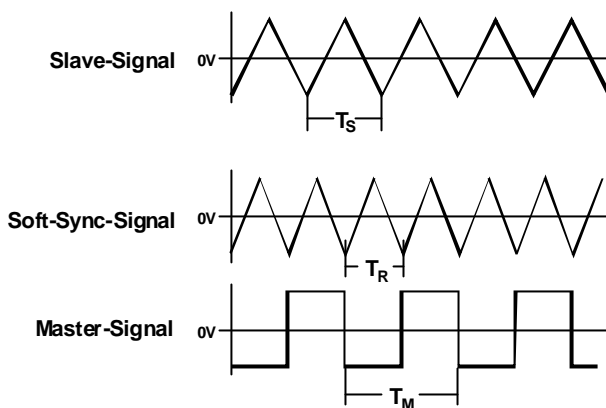
Fig. 14: Soft sync on the A-111
