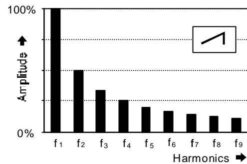
Fig. 1: Harmonic spectrum of a sawtooth
